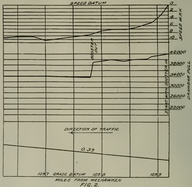
DYNAMOMETER RECORD OF BOOSTER LOCOMOTIVE ON THE CATSKILL GRADE
